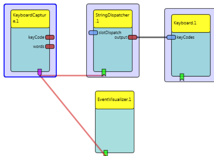
Figure 6: Model with three selected components
