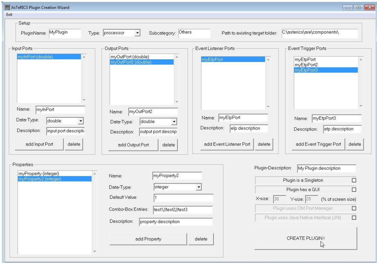
Figure 12: Screenshot of the AsTeRICS Plugin Creation Wizard
