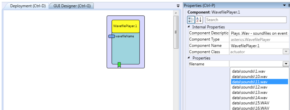
Figure 7: Plugin with Dynamic Property
